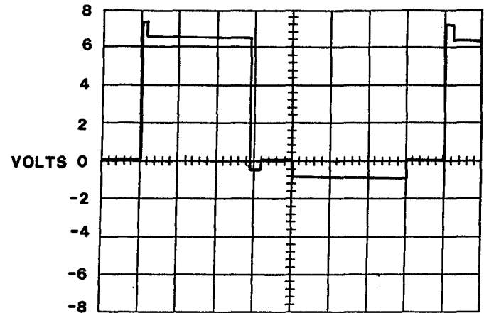
TIME = 5 MICROSECONDS/DIVISIONS 2-8(D)
