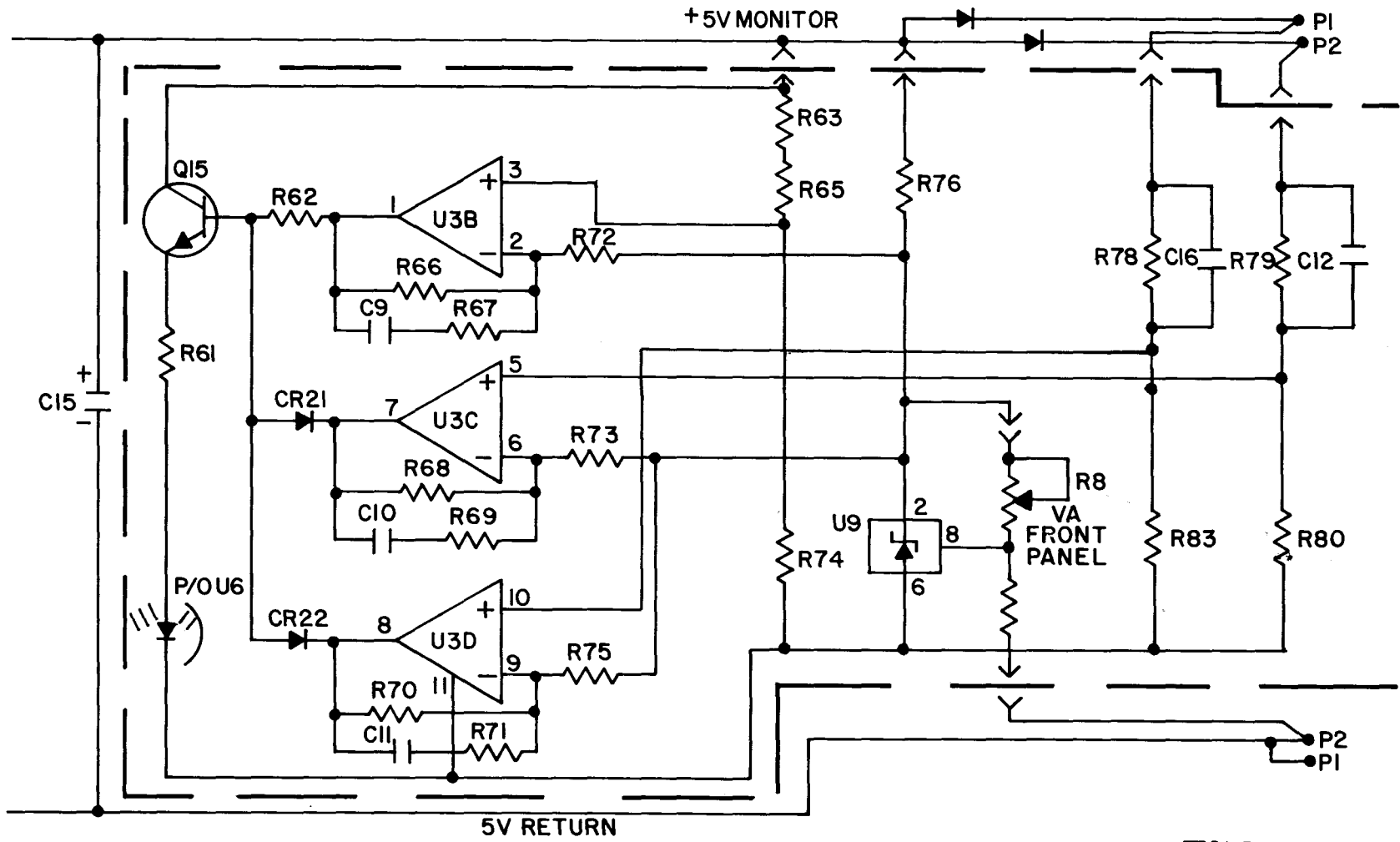
Figure 1-5. Regulator Loop.
