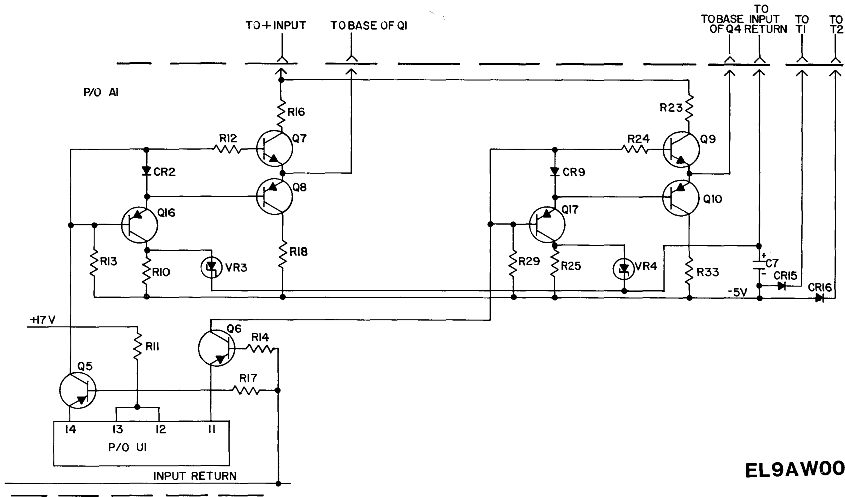
Figure 1-8. Drive Circuits
