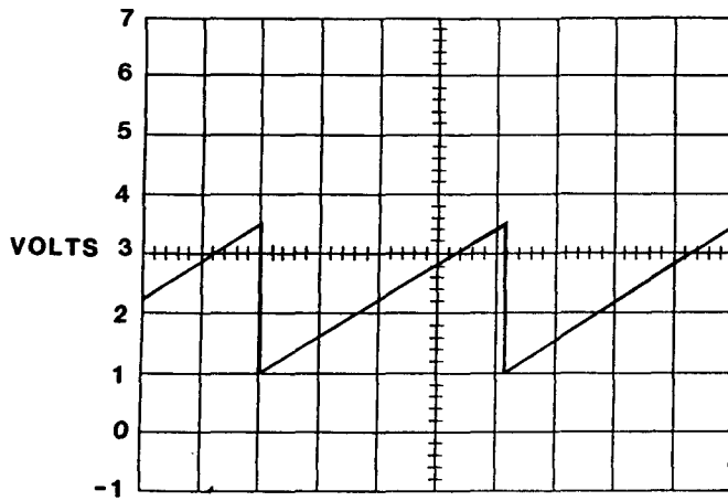
TIME = 5 MICROSECONDS/DIVISIONS 2-8(A)
