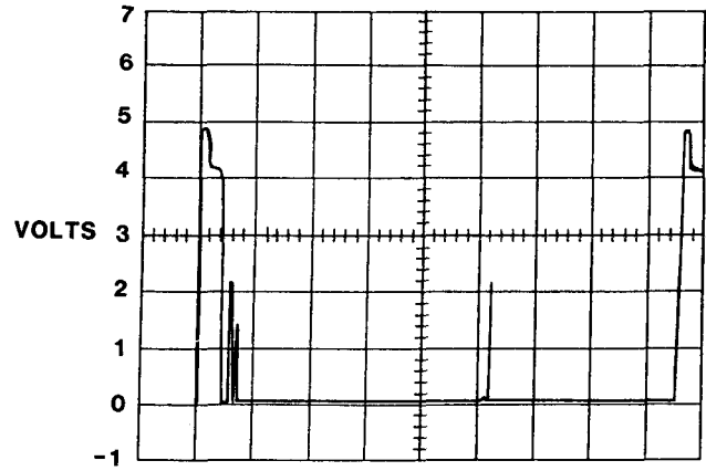
TIME = 5 MICROSECONDS/DIVISION 2-8(G)
