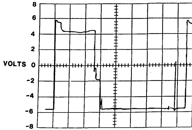
TIME = 5 MICROSECONDS/DIVISION 2-8(E)
