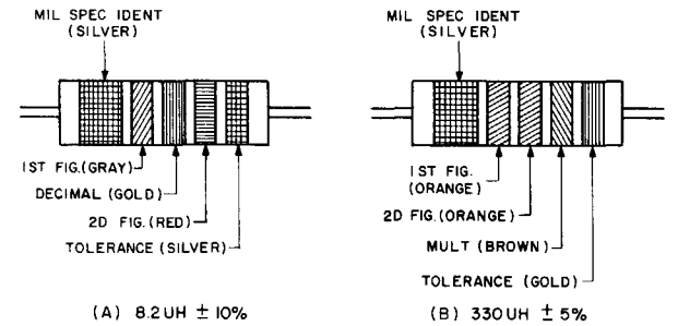
COLOR CODING FOR TUBULAR ENCAPSULATED R.F. CHOKES. AT A, AN EXAMPLE OF THE CODING FOR AN 8.2UH CHOKO IS GIVEN. AT B, THE COLOR BANDS FOR A 330UH INDUCTOR ARE ILLUSTRATED.
