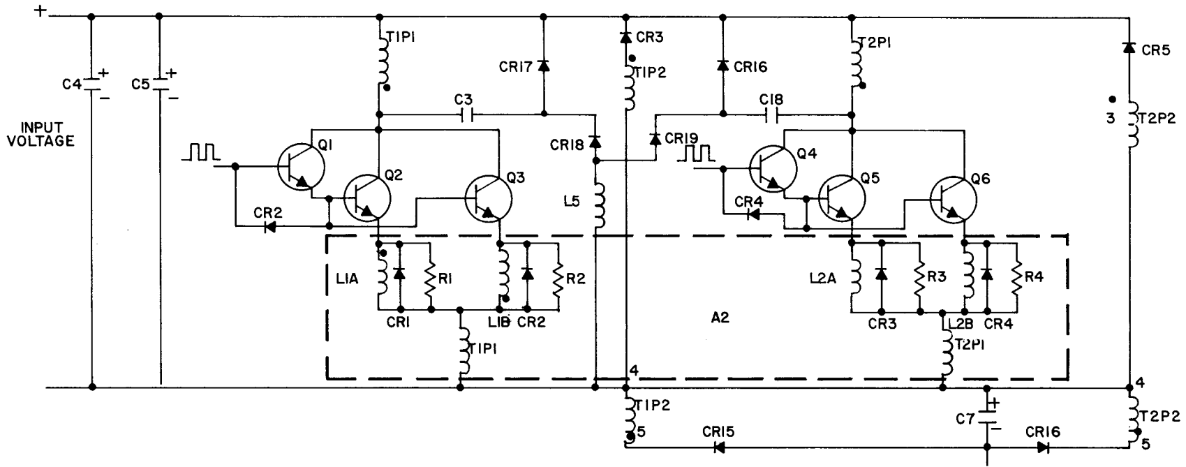
Figure 1-3. EMI Filter and Related Components and 20 KHz Switching Converter.
