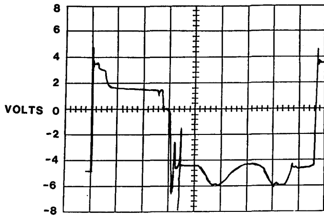
TIME = 5 MICROSECONDS/DIVISION 2-8(F)
